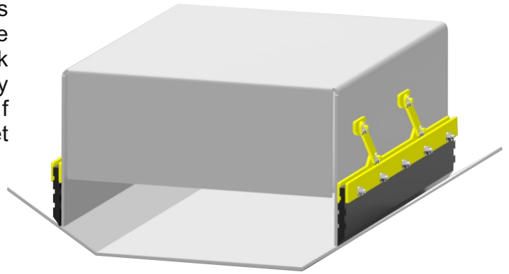
Optic Image after installation of BMD BHARAT SELF ADJUSTED SKIRT SEAL SYSTEM
